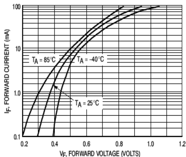
Figure 4. Forward Voltage
